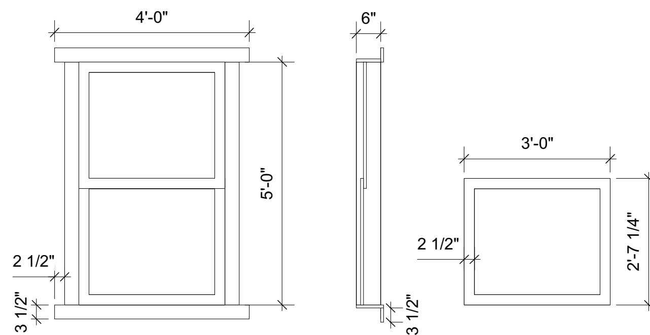
2 DS Window- Build 2 Scale: 1/2" = 1'-0"
