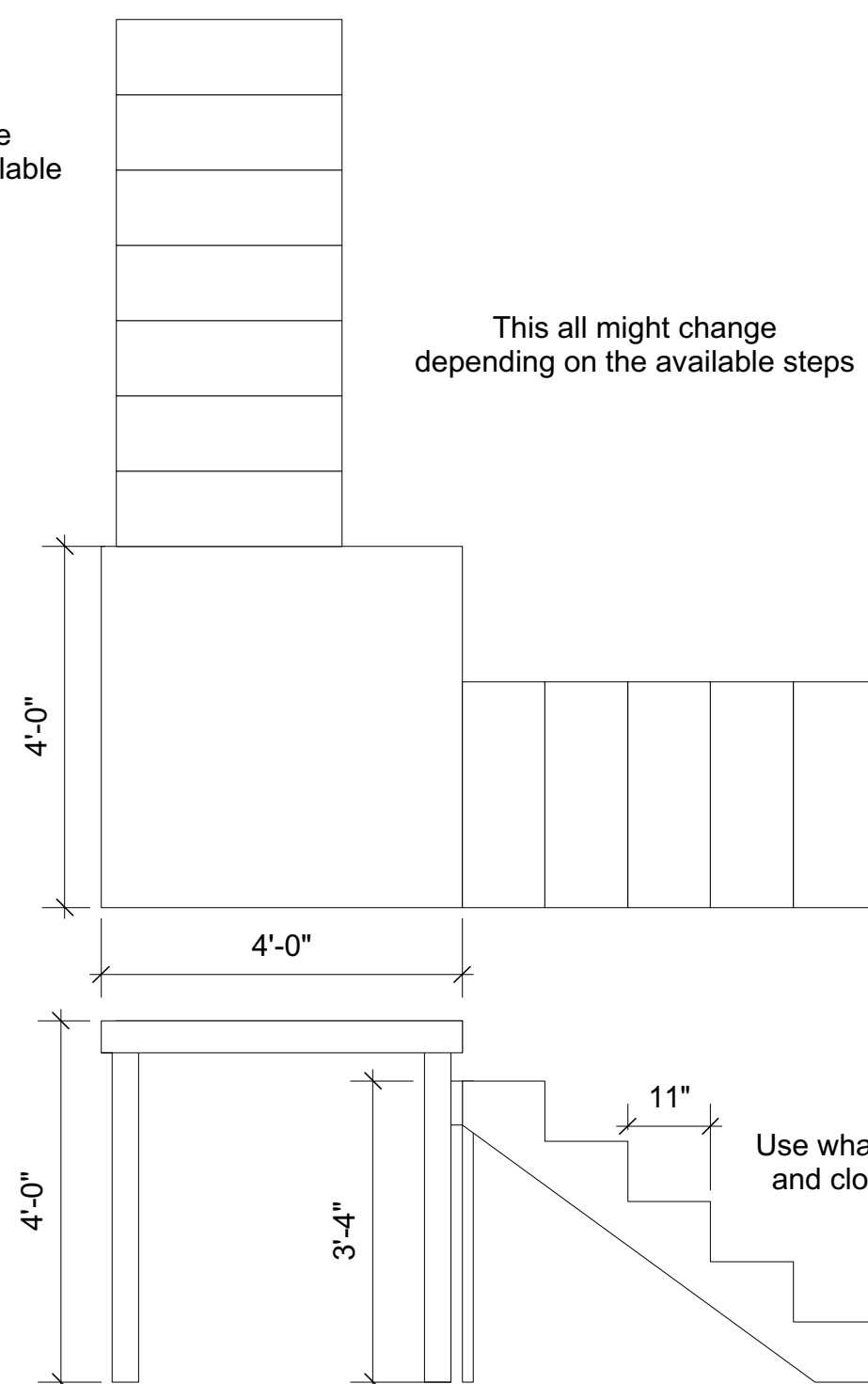
4 In-House Stair Units Scale: 1/2" = 1'-0"
